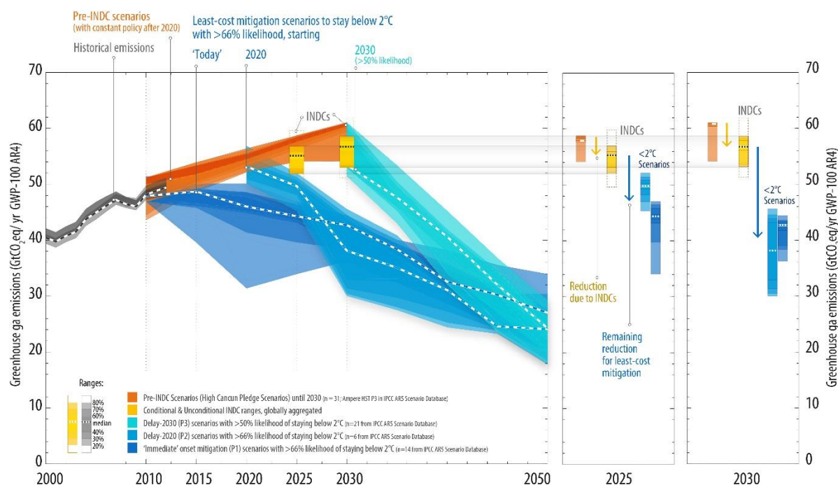
Figure 2 Comparison of global emission levels resulting from the intended nationally determined contributions in 2025 and 2030 with other trajectories
